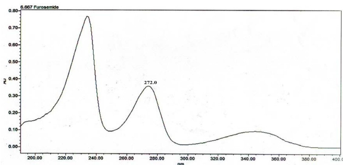
Figure 2. UV spectrum of Furosemide in mobile phase.
