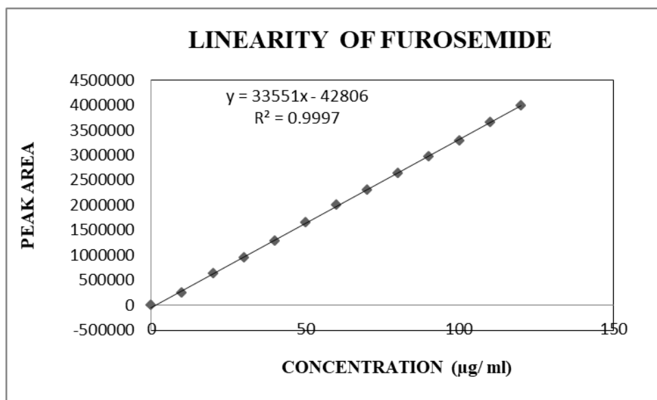
Figure 5. Calibration curve of Furosemide.
