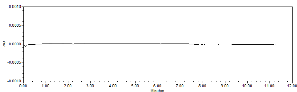
Figure 6. Chromatogram for blank.
