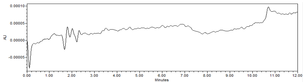
Figure 7. Chromatogram for matrix solution.
