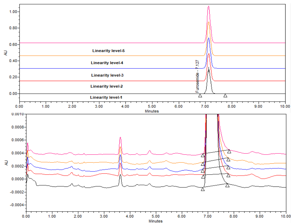
Figure 4. Linearity chromatogram of Furosemide.
