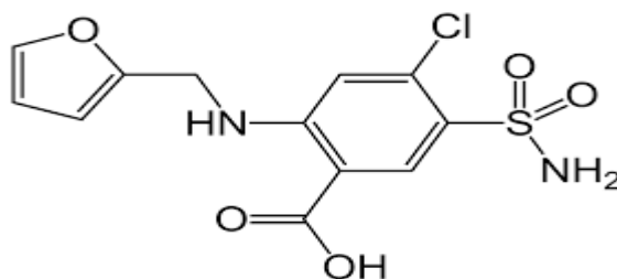
Figure 1. Molecular structure of Furosemide.
