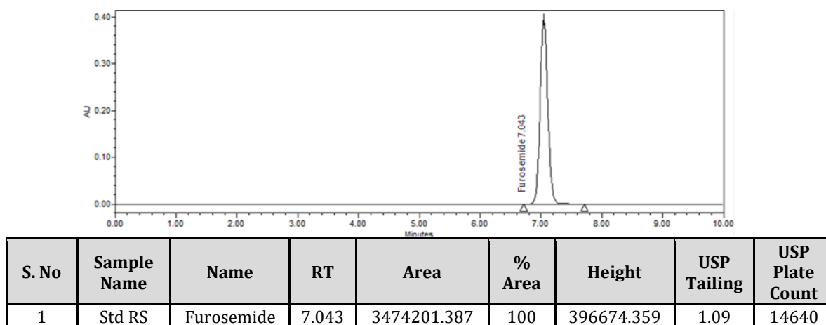
Figure 3. Optimized chromatogram of Furosemide.
